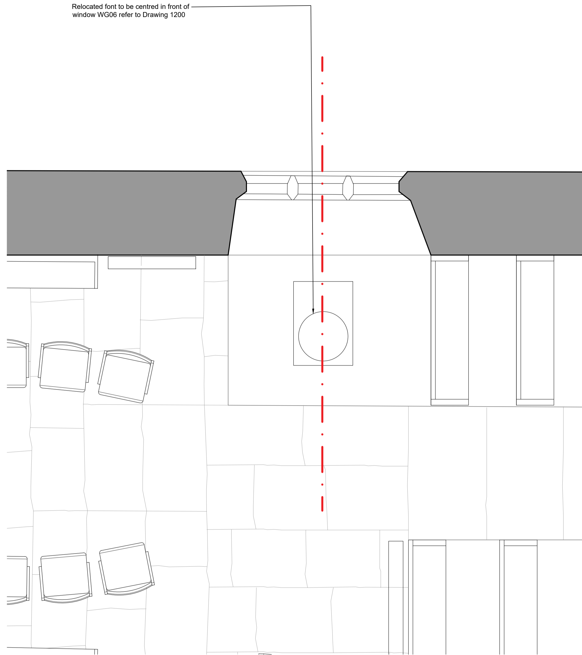
Detailed Plan of the relocated Font as proposed Scale 1:20 @ A1
