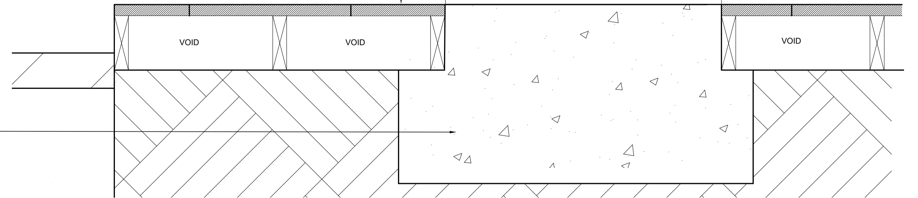
Detailed Section of the Font - As Proposed Scale 1:5 @ A1
